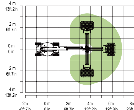
Range of Jib Swing Motion ZA10RJE
