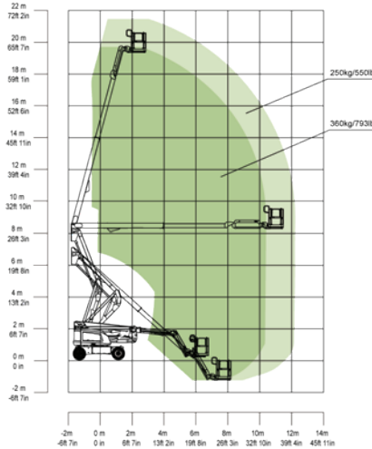
Range of Motion ZA20JERT/ZA20JERT-Li
