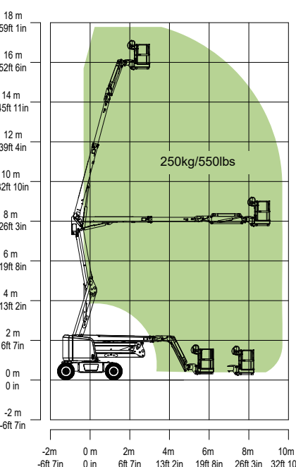
Range of Motion ZA16JERT/ZA16JERT-Li
